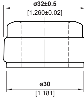
FINISH DETAIL - 2:1
