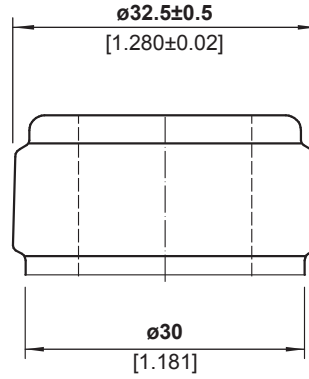
FINISH DETAIL - 2:1
