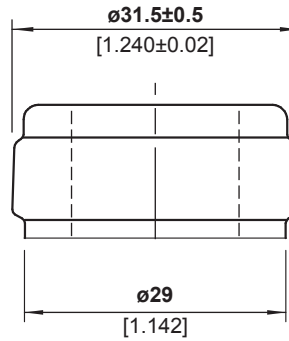
FINISH DETAIL - 2:1
