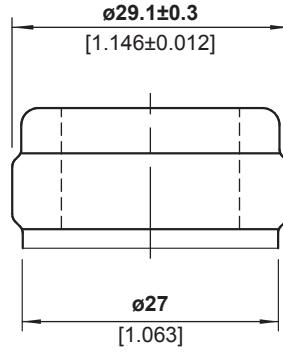
FINISH DETAIL - 2:1
