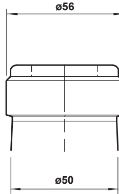
FINISH DETAIL - 2:1
