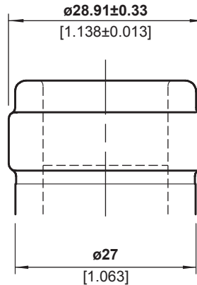
FINISH DETAIL - 2:1
