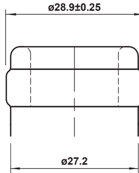
FINISH DETAIL - 2:1
