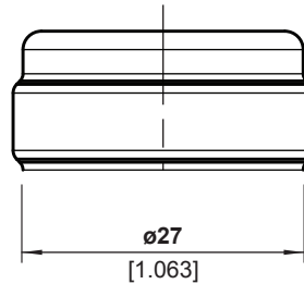
FINISH DETAIL - 2:1
