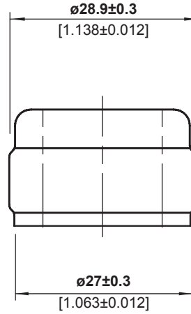
FINISH DETAIL - 2:1
