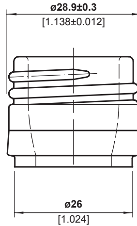
FINISH DETAIL - 2:1
