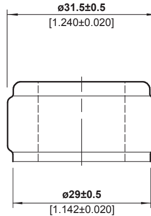
FINISH DETAIL - 2:1
