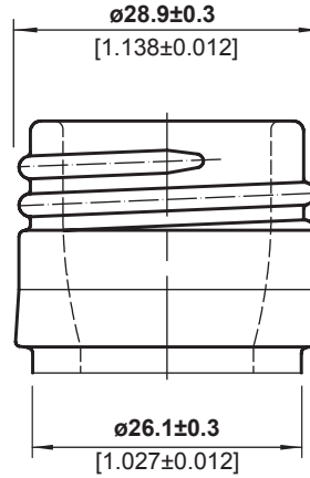
FINISH DETAIL - 2:1
