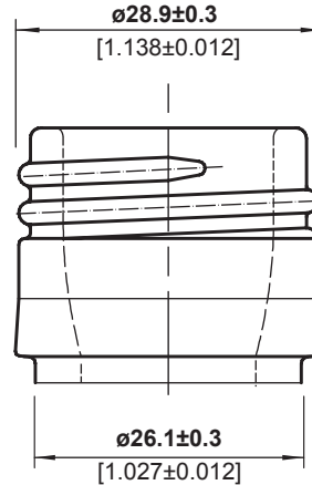
FINISH DETAIL - 2:1
